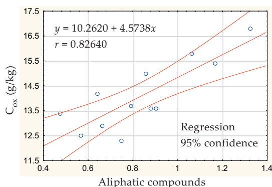
Figure 4. Correlation aliphatic compounds vs. C_{ox} (autumn 2003)
