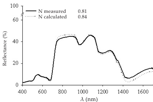
Figure 9. Spectral reflectance at different wavelengths ( \lambda ) of oilseed rape canopy ( -N ) and reflection index NDVI (given as numbers) at May 28, 2003 measured with field configuration (line) and re-calculated after equation 1 (dotted) ( n = 60 )
