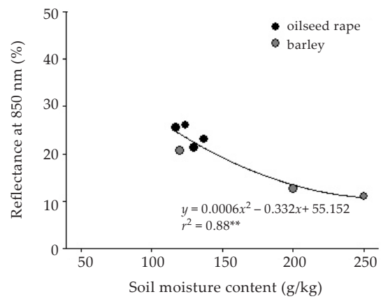
Figure 7. Relation between soil reflection values at 850 nm and soil moisture content during vegetation of winter oilseed rape (black) and barley (grey) ( n = 7 , ** indicates significance at the P < 0.01 level)
