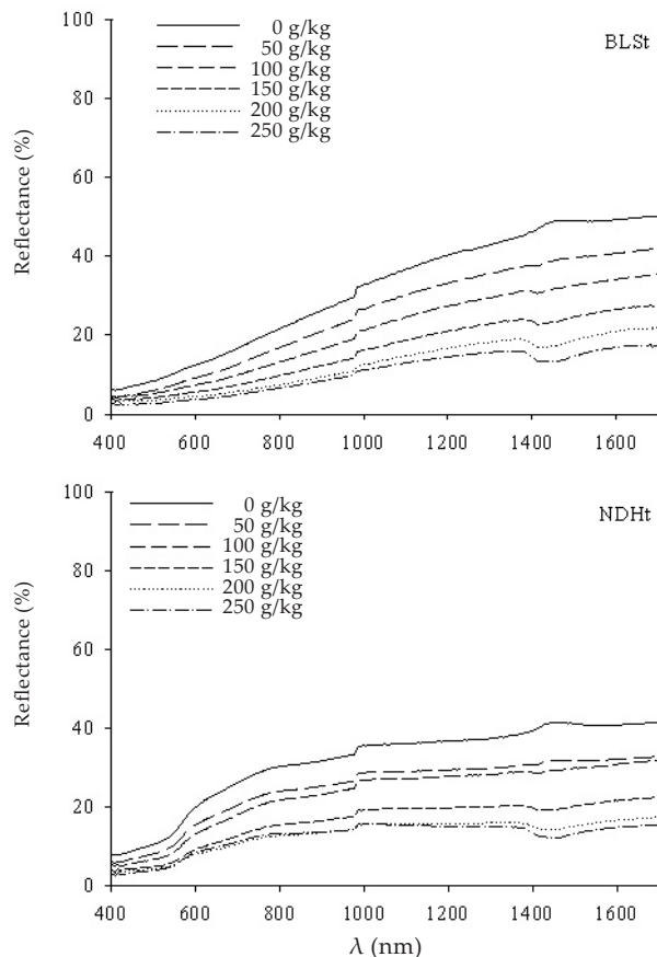
Figure 4. Soil reflectance at different wavelengths ( \lambda ) of two soils as affected by varied soil moisture contents (g/kg) measured with laboratory configuration OMK ( n = 20 )
