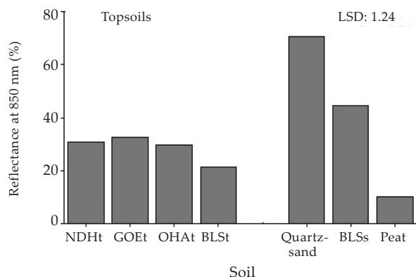
Figure 2. Reflection values at 850 nm measured with laboratory configuration OMK as affected by soil type and origin; all soils are significantly different at P < 0.05 (Tukey, n = 20 )
