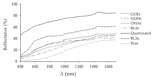
Figure 1. Soil reflectance at different wavelengths ( \lambda ) measured with laboratory configuration OMK as affected by soil type and origin ( n = 20 )
