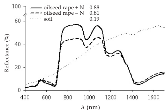
Figure 8. Spectral reflectance at different wavelengths ( \lambda ) of bare soil and oilseed rape canopies (–N, +N) and reflection index NDVI (given as numbers) at May 28, 2003 with the field configuration ( n = 60 )
