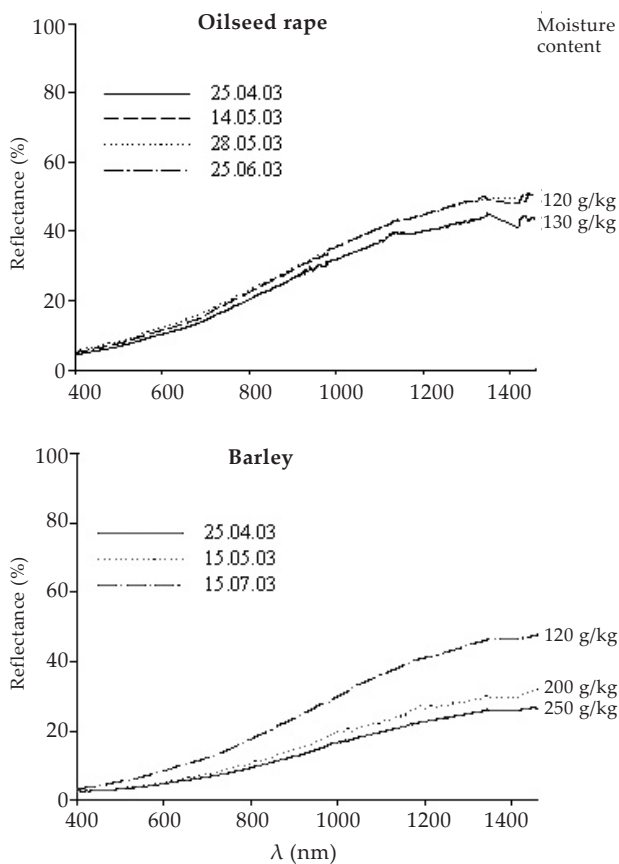
Figure 6. Soil reflectance at different wavelengths ( \lambda ) as affected by soil moisture content of the topsoil (0–20 cm) during vegetation of winter oilseed rape and barley measured with field configuration ( n = 15 )
