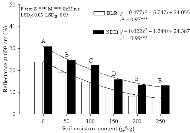
Figure 5. Reflection values at 850 nm of two different agricultural soils (S): Bad Lauchstaedt (white) and Nordhausen (black) as affected by varied soil moisture contents (M) measured with laboratory configuration OMK (means followed by different letters are significantly different at P < 0.05 , Tukey, n = 20 ) and relations between reflectance at 850 nm and soil moisture content ( n = 20 , *** indicates significance at the P < 0.001 level)
