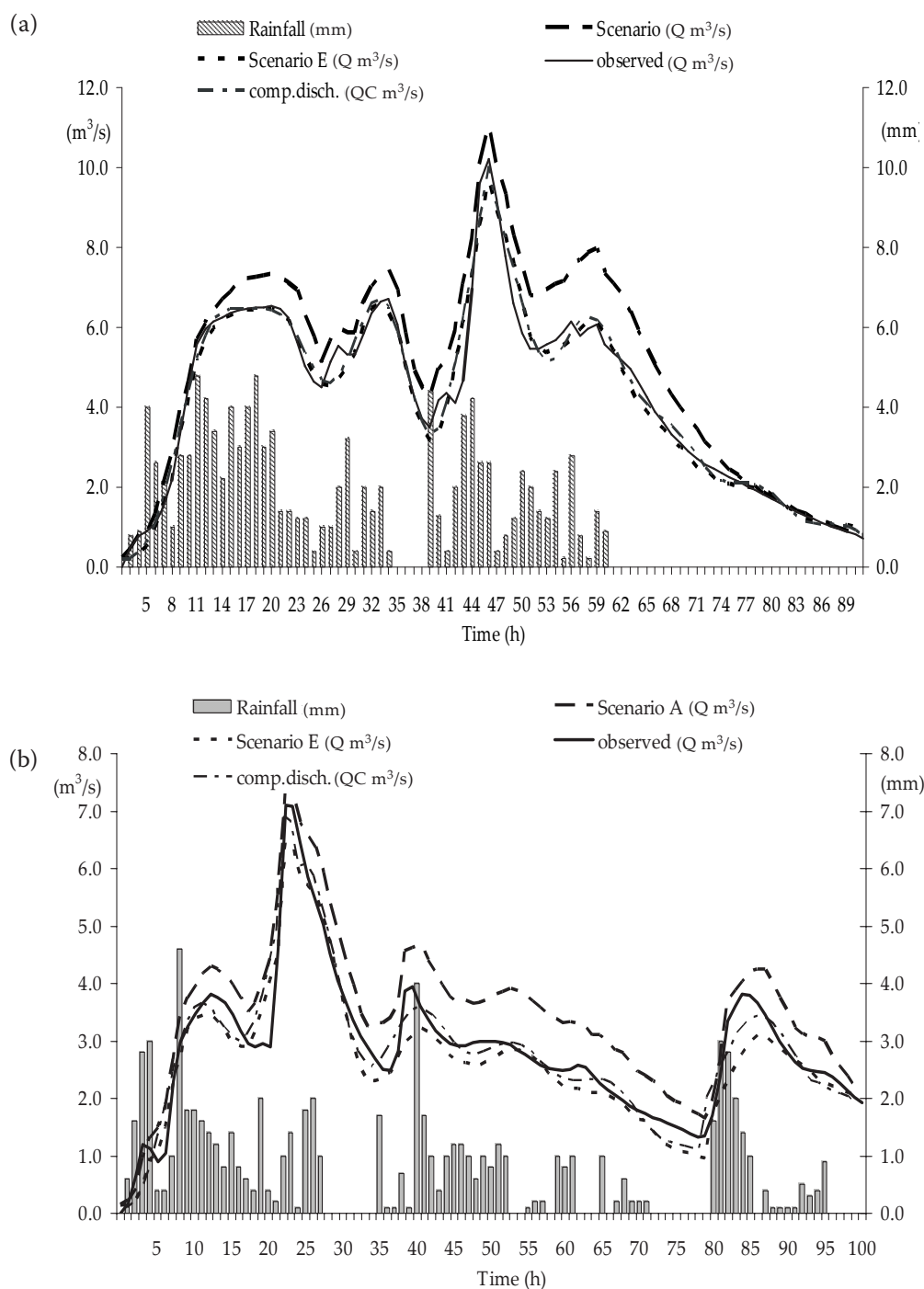
Figure 2. Comparison of ordinates of observed and reconstructed discharges (including scenarios) on the Všeminka catchment
