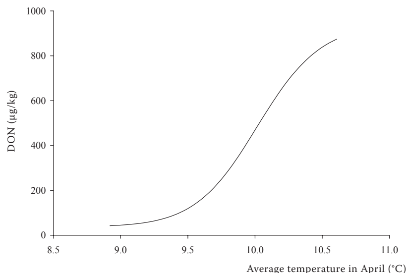
Figure 5. Response graph of input variable average temperature in April for winning neural network ZRNS 5:5-12-2-1:1, for prediction of DON content when other input variables are fixed
