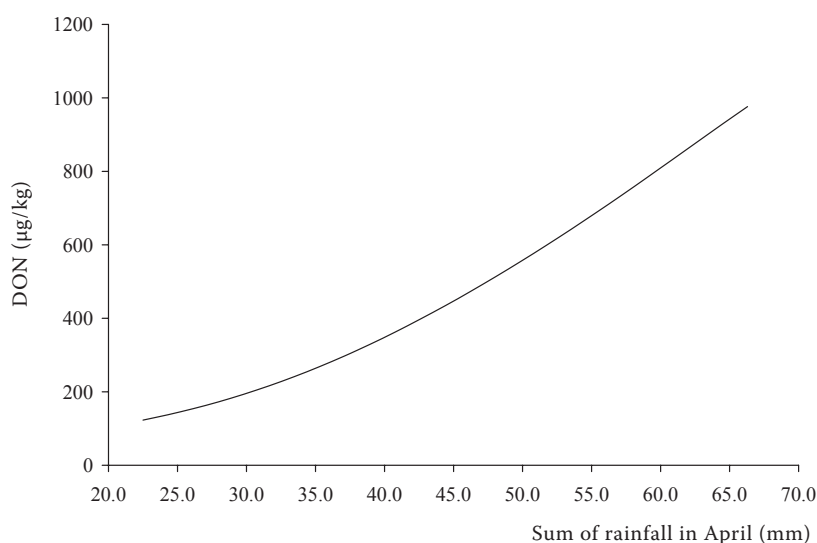
Figure 6. Response graph of input variable sum of rainfall in April for winning neural network ZRNS 5:5-12-2-1:1, for prediction of DON content when other input variables are fixed
