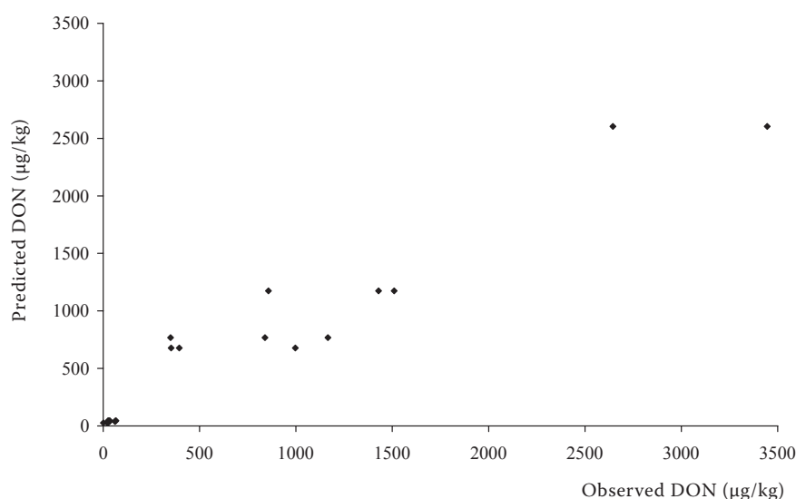
Figure 3. Graph of fit between observed and predicted (using neural network with weather input variables ZRNS 5:5-12-2-1:1) DON concentrations in grain
