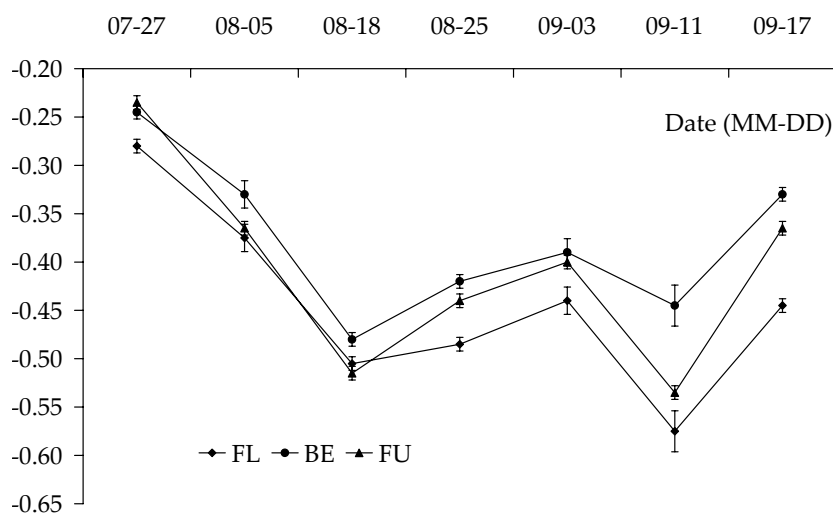
Figure 3. Variation of leaf water potential during the growing season of summer maize
