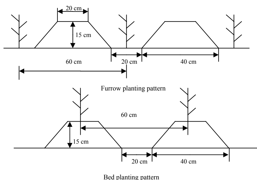
Figure 1. The schematic diagram showing furrow and bed planting patterns
