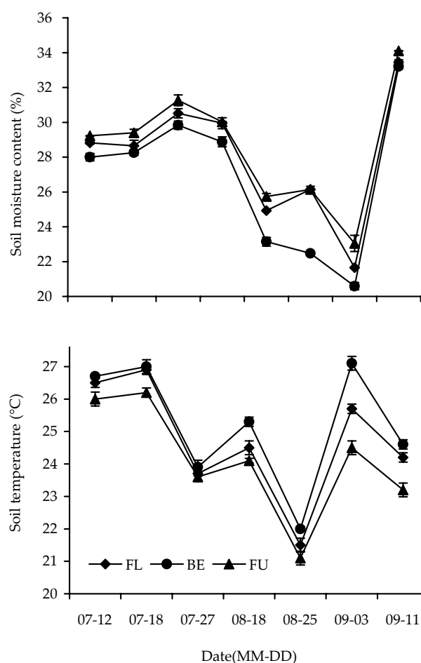
Figure 4. Variation of soil moisture content and soil temperature in the growing season of summer maize
