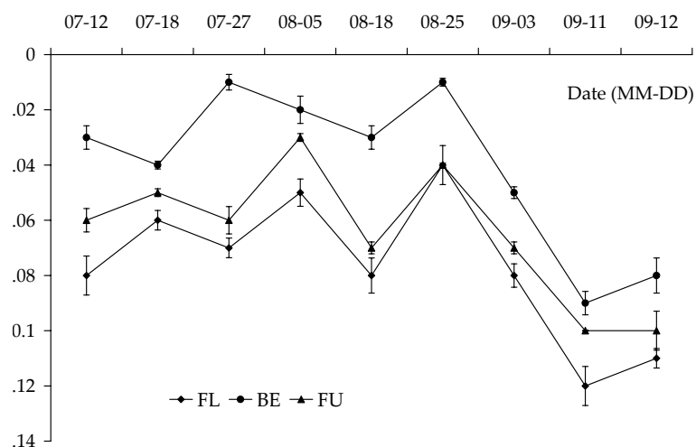
Figure 2. Variation of soil water potential during the growing season of summer maize
