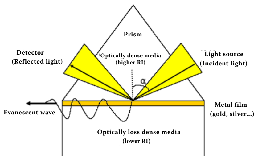
Figure 3. Schematic of the SPR system in the Kretschmann configuration
