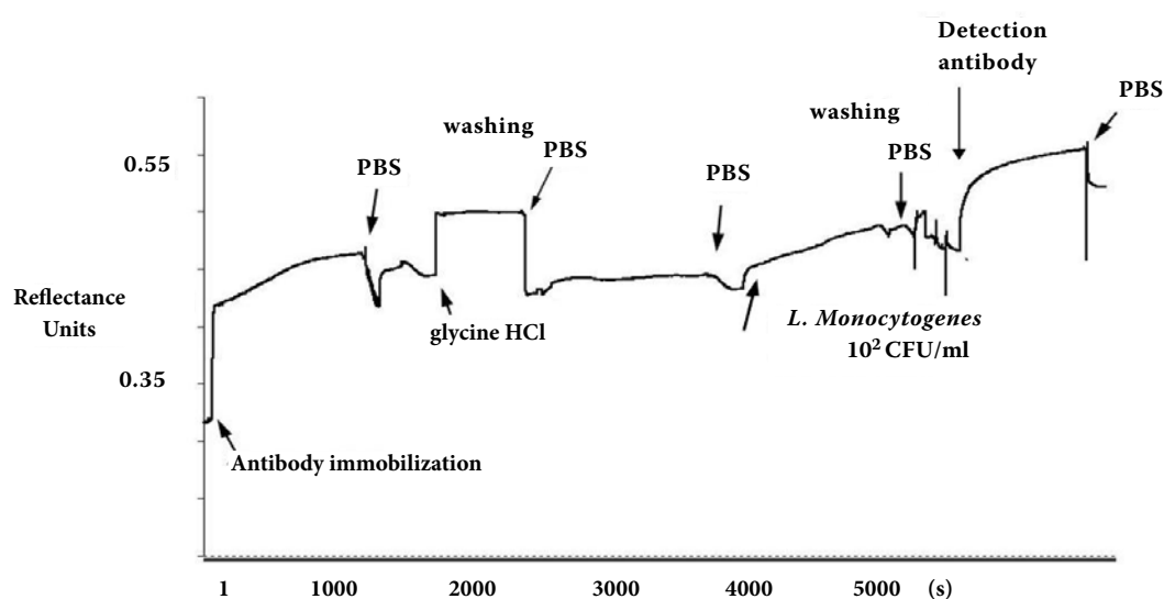
Figure 4. The SPR sensogram for the detection of Listeria monocytogenes ( 10^2 CFU/ml) in PBS buffer, monitored over time. On the y axis detection signal expressed in reflectance units
