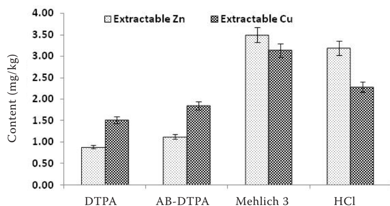
Figure 1. Comparative extractability of extractants for zinc and copper
