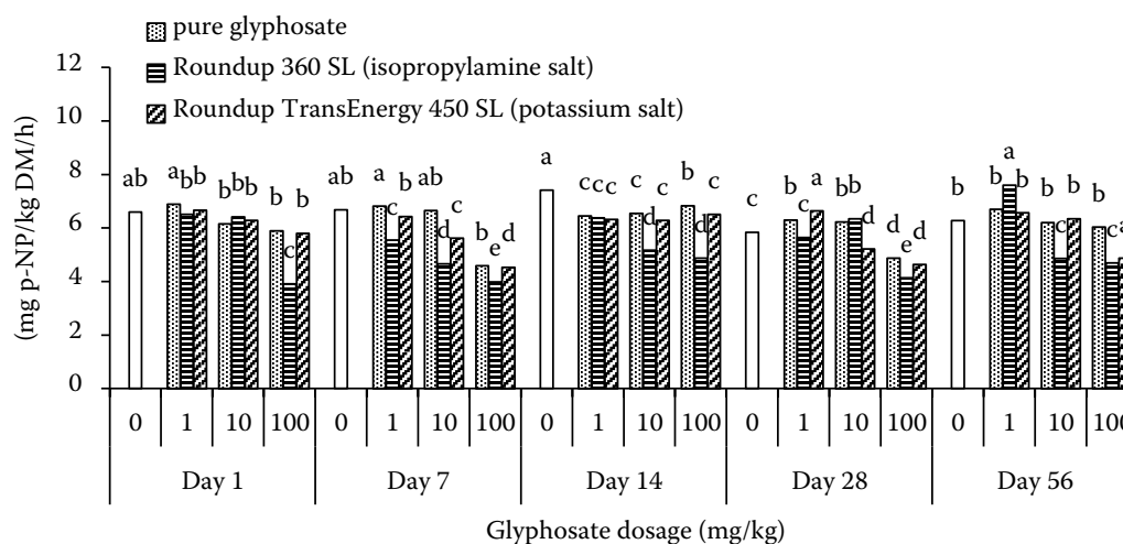
Figure 3. Phosphodiesterase activity in soil treated with glyphosate and its formulations. Values denoted with the same letters within the day of experiment do not differ statistically ( P < 0.05 ); p-NP – p-nitrophenol; DM – dry matter
