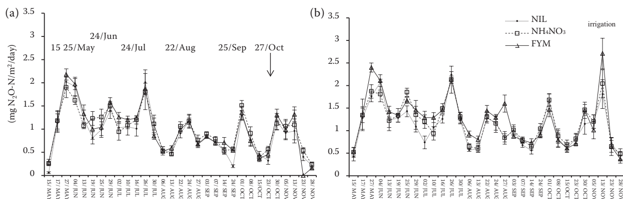
Figure 1. \text{N}_2\text{O} -N emissions from the soils long-term treated with (a) mineral and (b) manure fertilizers (FYM) upon experimental application of ammonium nitrate and manure and under NIL (non-treated) treatment
