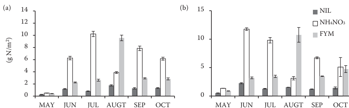
Figure 4. Mineral-N soil leaching from the soils long-term treated with (a) mineral and (b) farmyard manure (FYM) fertilizers upon experimental application of \text{NH}_4\text{NO}_3 , FYM and under NIL (non-treated) treatment
