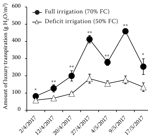
Figure 3. The amount of luxury transpiration under different irrigation schedules. * P < 0.05 ; ** P < 0.01 ; FC – field capacity
