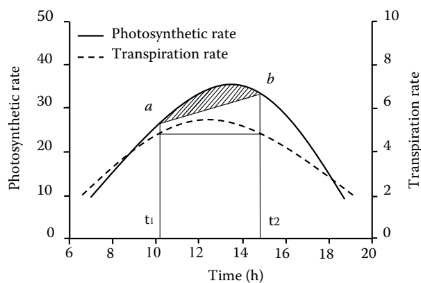
Figure 1. The diagram of luxury transpiration calculations ( t_1 – starting time of luxury transpiration; t_2 – ending time of luxury transpiration)
