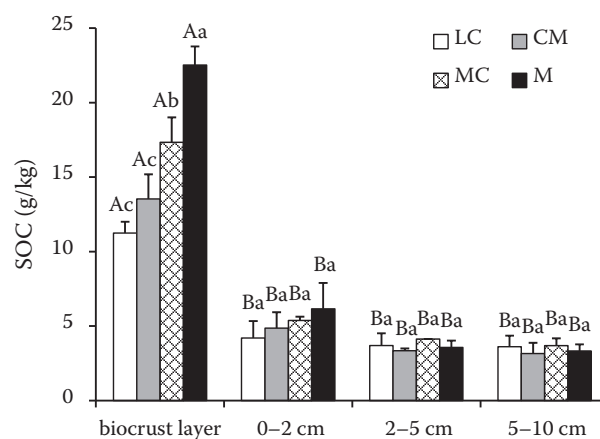
Figure 1. Soil organic carbon (SOC) content in four biocrusts at different soil layers. Values are in the form of mean \pm standard deviation ( n = 3 ). Different upper-case letters above the bars indicate significant differences between different soil layers of the same biocrust types. Different lower-case letters above the bars indicate significant differences between different biocrusts of the same soil layers ( P < 0.05 ). LC – light cyanobacteria biocrust; CM – cyanobacteria mixed with sparse moss; MC – moss mixed with sparse cyanobacteria; M – moss crust
