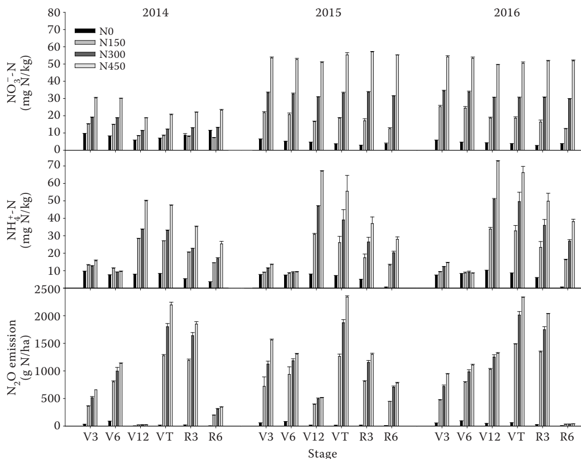
Figure 4. Nitrate nitrogen ( \text{NO}_3^-\text{-N} ) and ammonium nitrogen ( \text{NH}_4^+\text{-N} ) at 0–20 cm depth, and accumulative \text{N}_2\text{O} emissions from critical maize stages in the N0, N150, N300, and N450 treatments. Vertical bars denote the standard error of the means ( n = 3 ). N0 – 0, N150 – 150, N300 – 300, N450 – 450 kg N/ha; V3 – trilobites period; V6 – six leaf stage; V12 – twelve leaf stage; VT – tasseling stage; R3 – ratooning buds; R6 – full ripeness period
