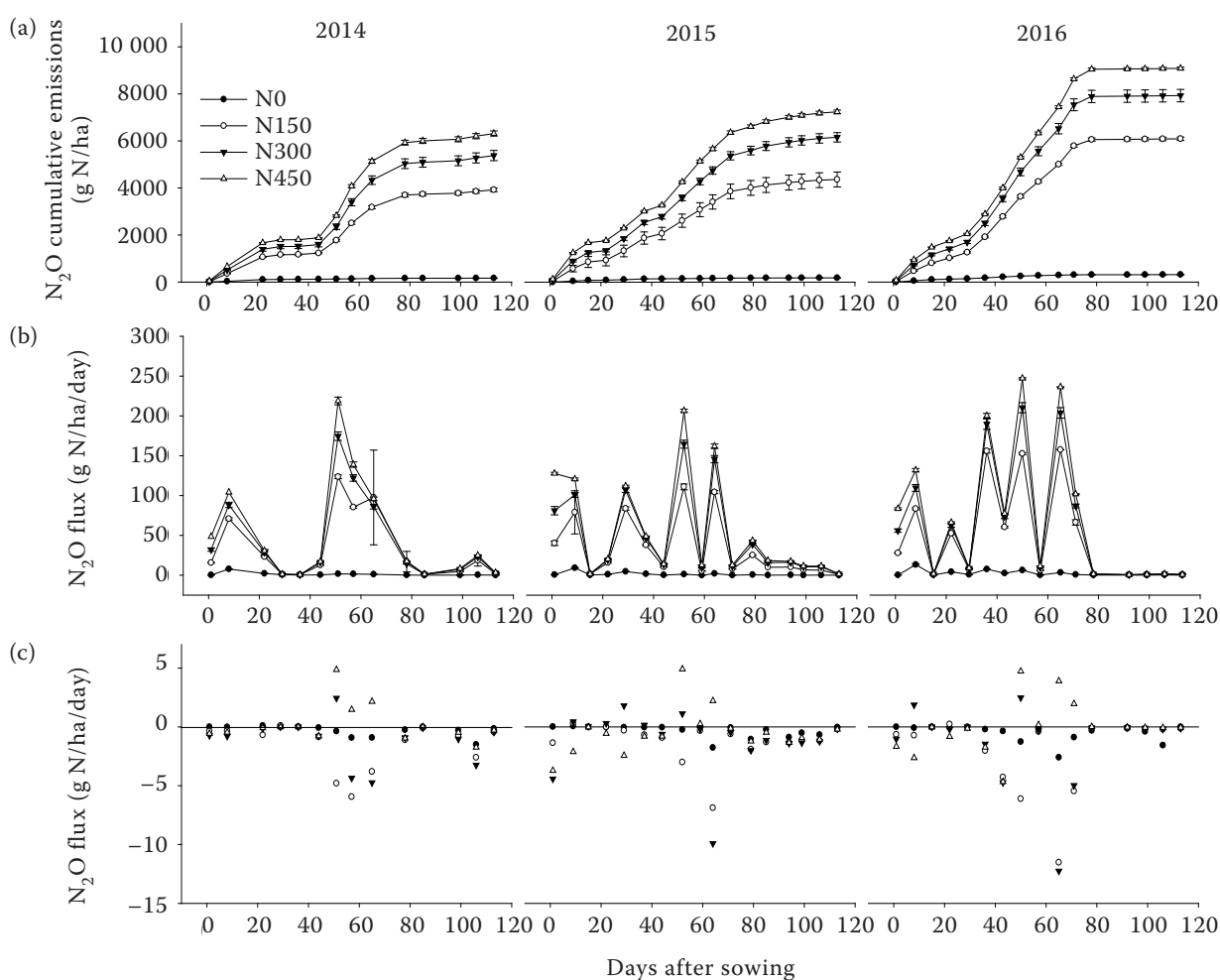
Figure 2. The planting maize field \text{N}_2\text{O} cumulative emissions (a); daily \text{N}_2\text{O} flux (b) and the daily \text{N}_2\text{O} flux difference between planting maize field and no planting maize fields (c) under different fertilizer rates during the maize growing season (2014–2016). N0 – 0, N150 – 150, N300 – 300, N450 – 450 kg N/ha
