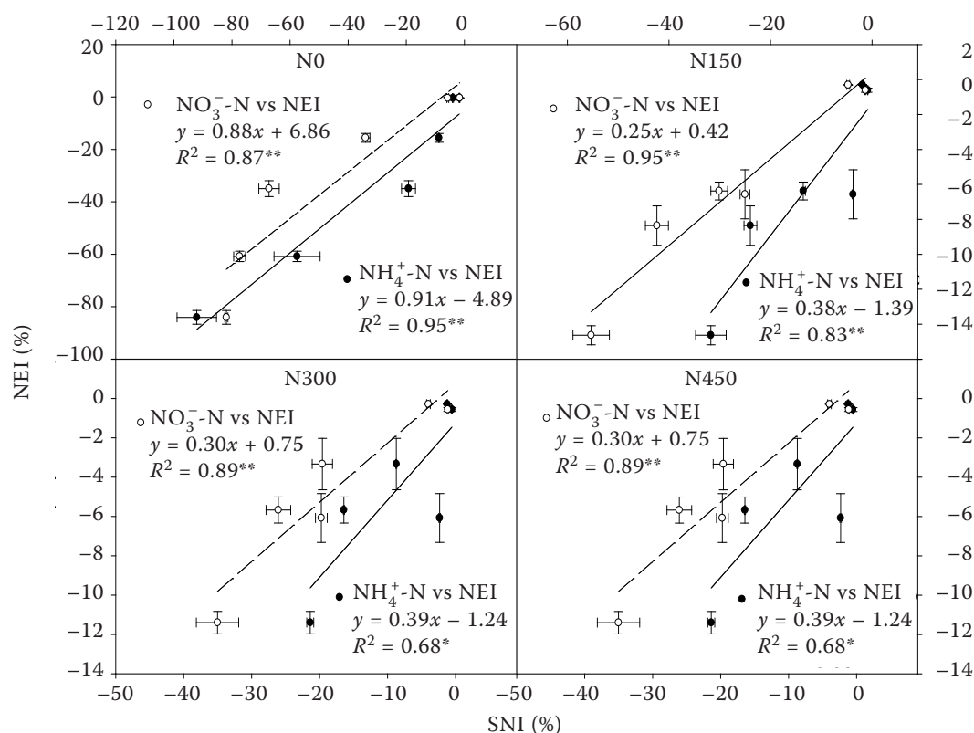
Figure 5. The correlation between the effect of nitrogen (N) on \text{N}_2\text{O} emission and soli N ( \text{NH}_4^+\text{-N} and \text{NO}_3^-\text{-N} ). N0 – 0, N150 – 150, N300 – 300, N450 – 450 kg N/ha; * P < 0.05 ; ** P < 0.01 ; *** P < 0.001 ; NEI – effect of maize growth on \text{N}_2\text{O} emission
